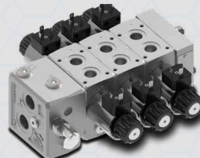
SDX060 Proportional bankable solenoid valve
