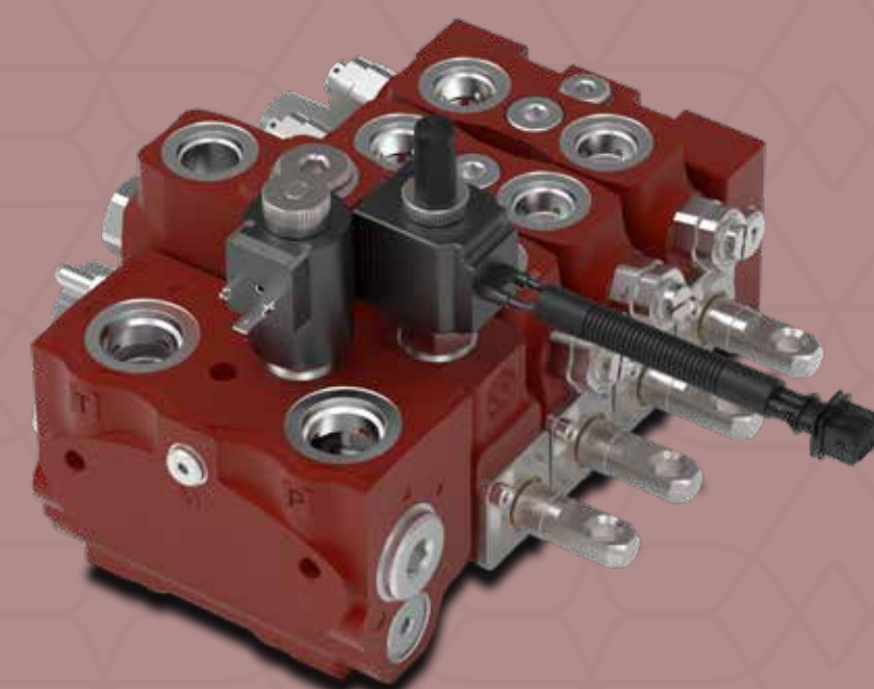
SD8 Sectional directional control valve
